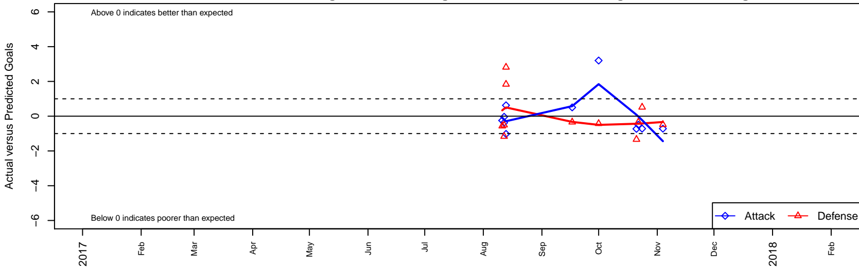
Sting SC Timbers Red G03 Dots are actual minus expected GF (blue circles) and GA (red triangles). Blue line is smoothed change in attack strength. Red is smoothed change in defense strength.
